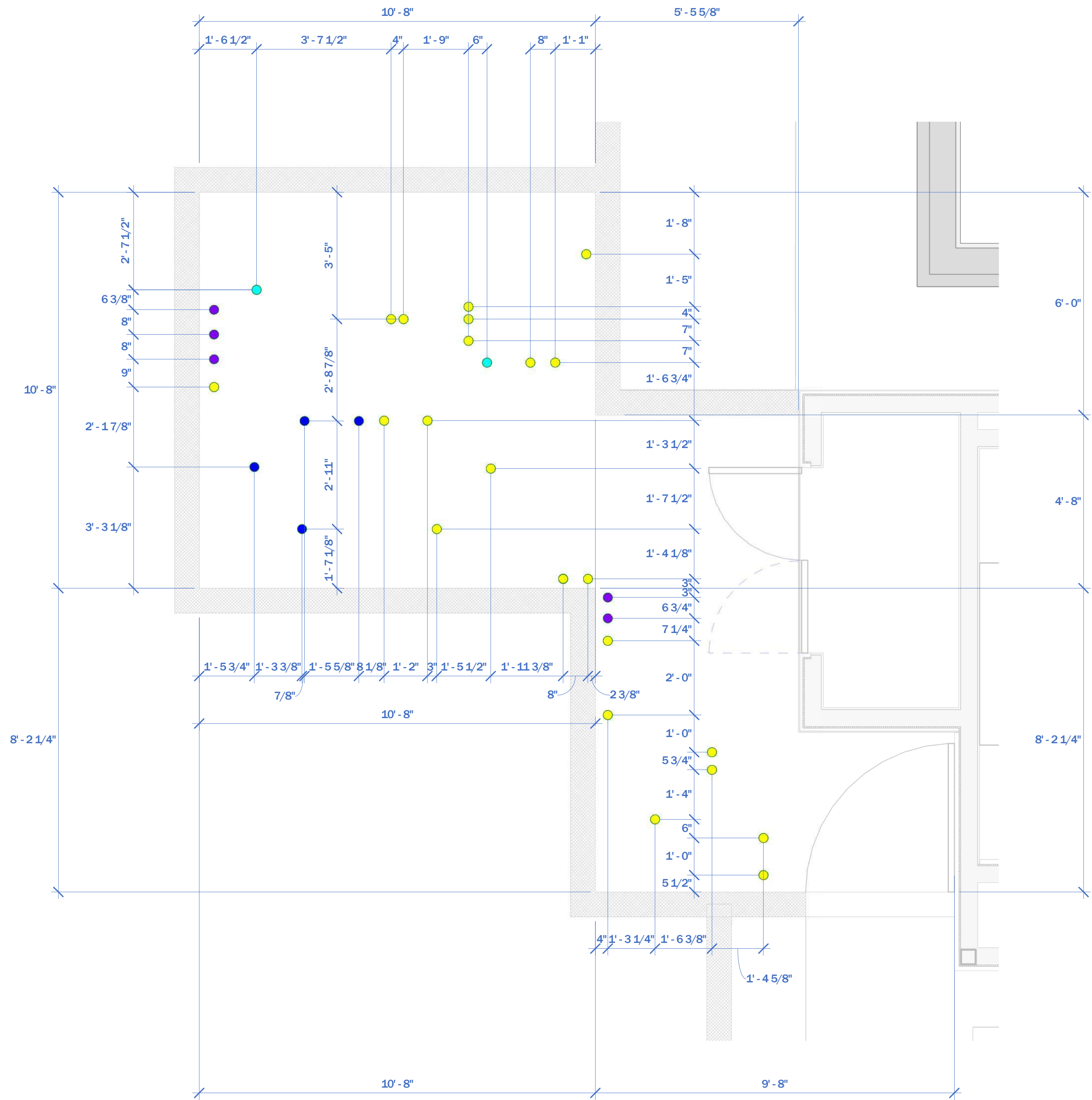
② EQUIPMENT PAD STUB-UP PIPING PLAN 1/2" = 1'-0"
