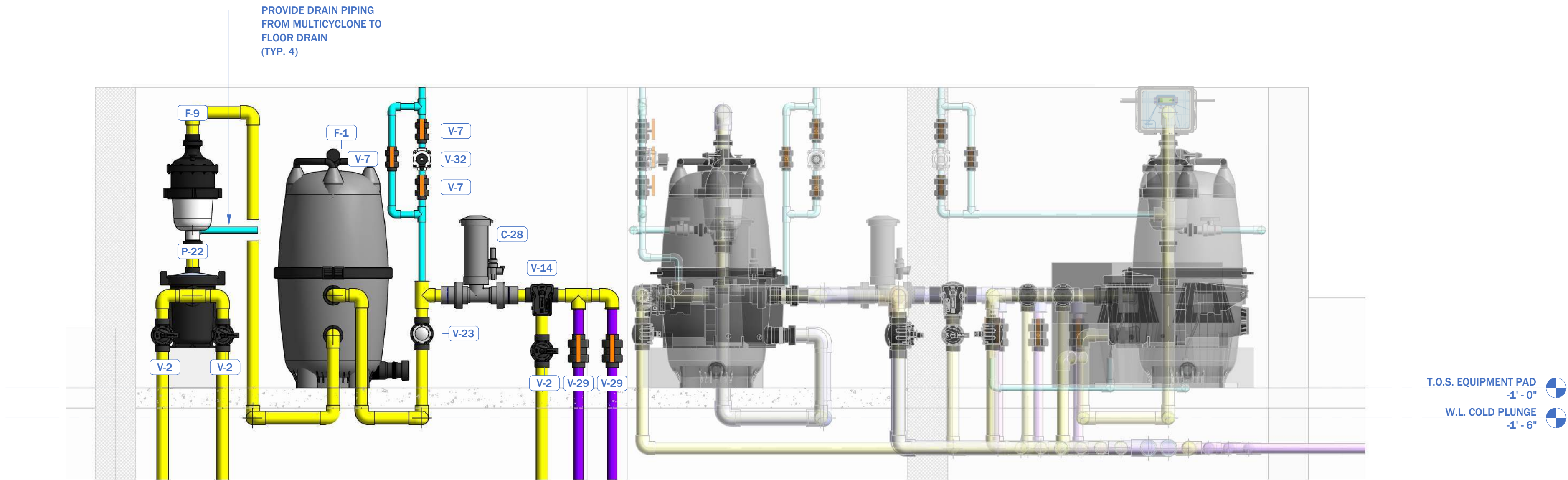
3 EQUIPMENT ELEVATION - FOUNTAIN 2 3/4" = 1'-0"
