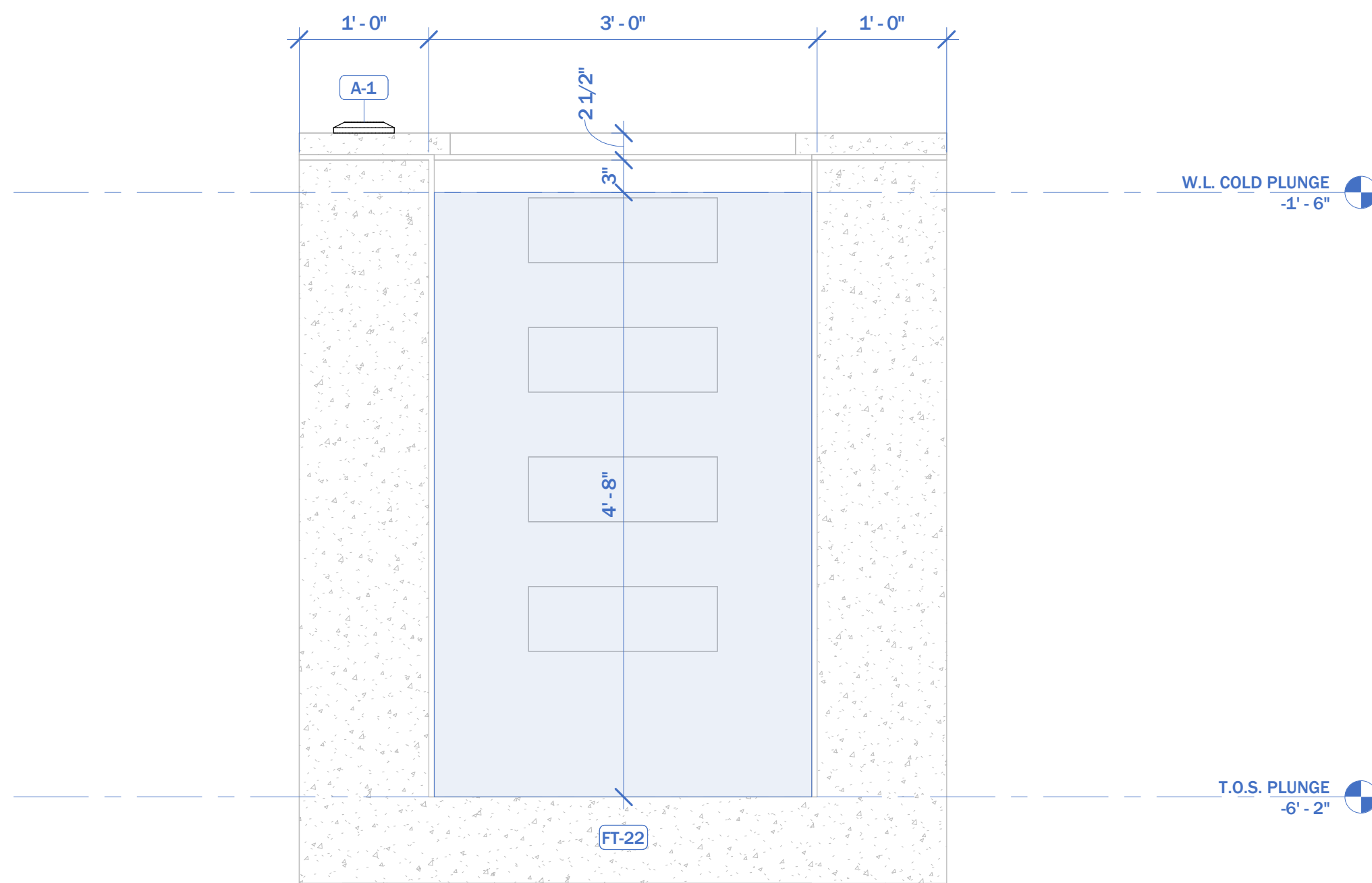
4 TRANSVERSE COLD PLUNGE SECTION 1" = 1'-0"
