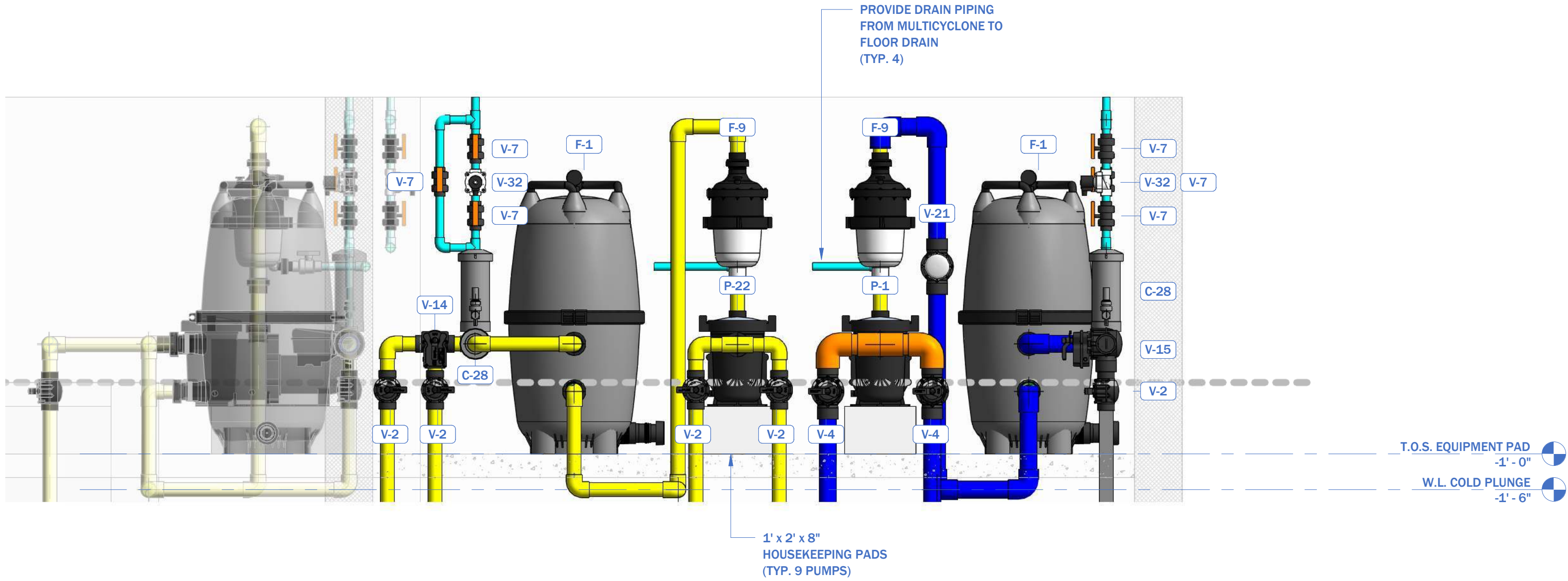
2 EQUIPMENT ELEVATION - WATER FEATURE, FOUNTAIN 1 3/4" = 1'-0"
