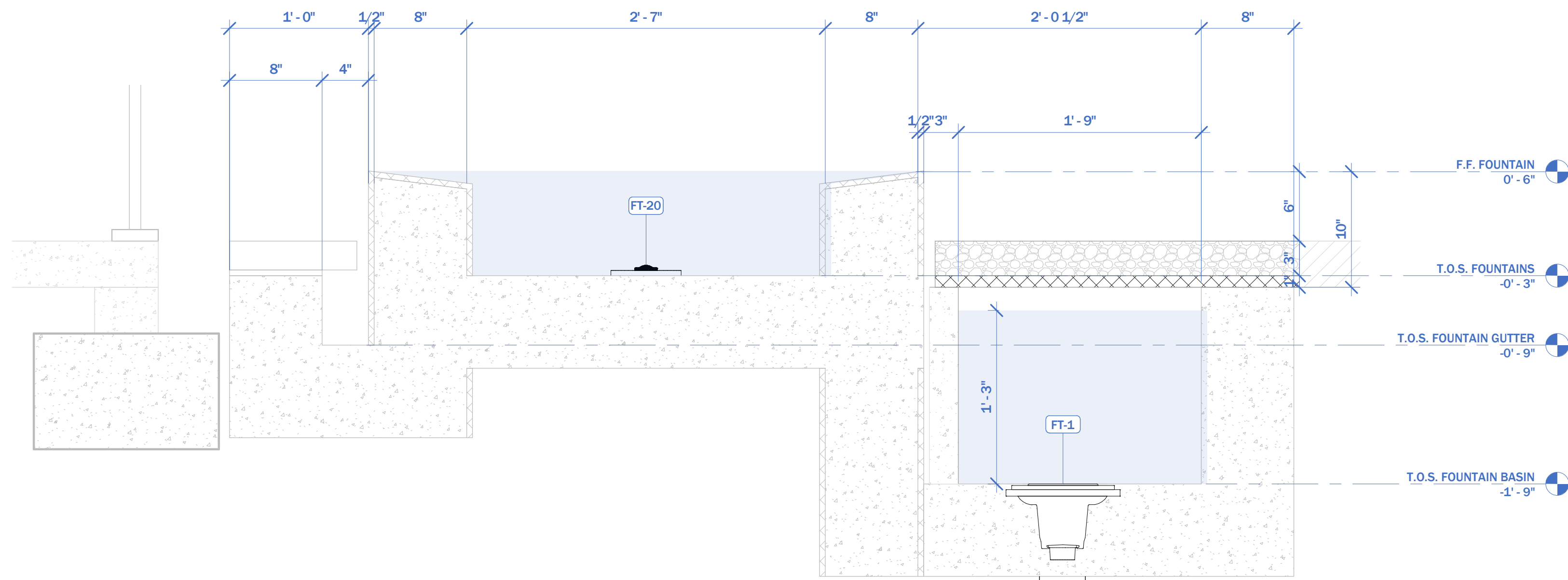
① TRANSVERSE FOUNTAIN & BASIN SECTION 1 1/2" = 1'-0"
