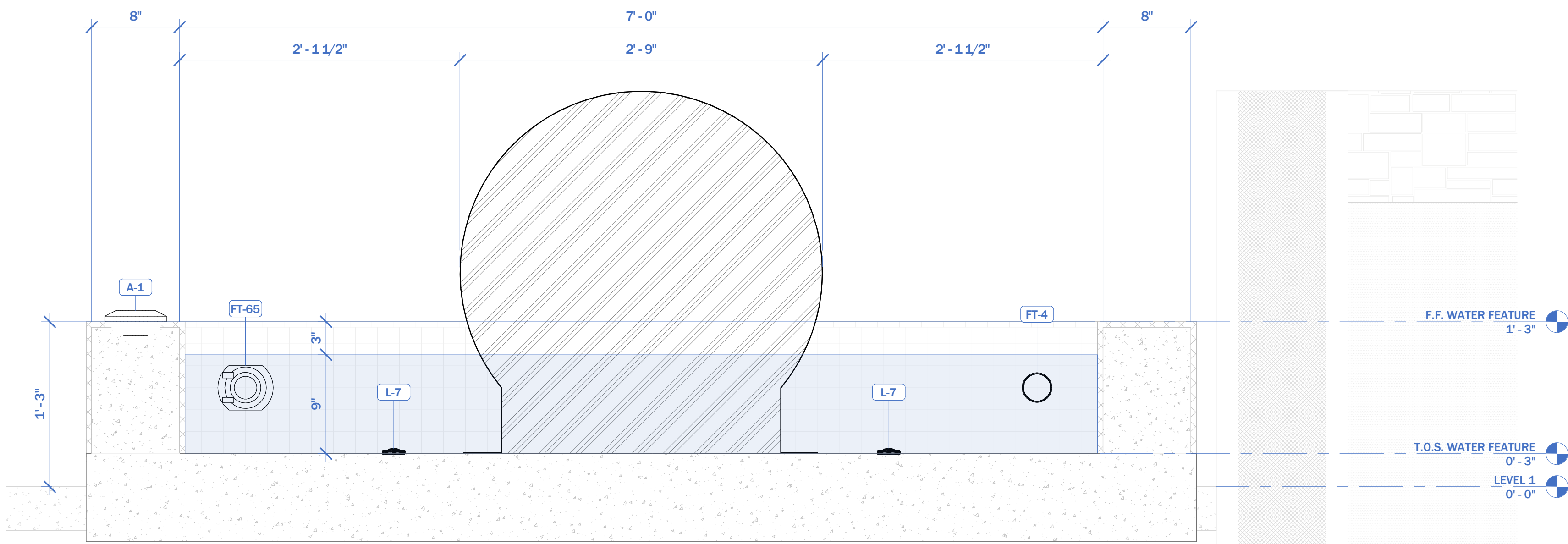
1 LONGITUDINAL WATER FEATURE SECTION 1 1/2" = 1'-0"
